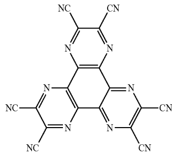
HAT-CN
