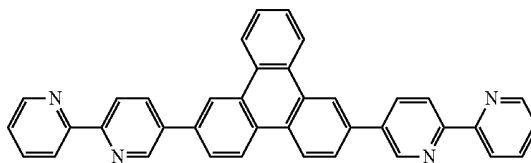
BPy-TP2
