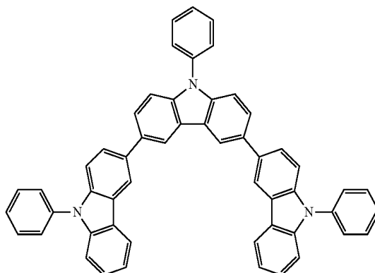
Tns-PCz
